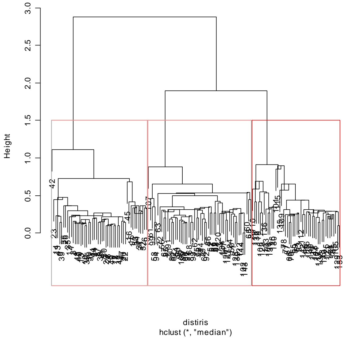
Cluster Dendrogram
